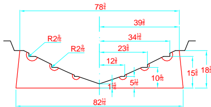
TRANSVERSAL SECTION "A" SECCION TRANSVERSAL "A"
