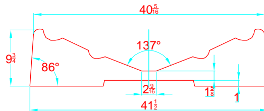
TRANSVERSAL SECTION "A" SECCION TRANSVERSAL "A"
