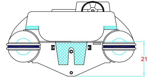
AFT VIEW VISTA TRASERA
