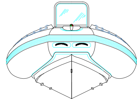
FORE VIEW VISTA FRONTAL MAIN PARTICULARS
