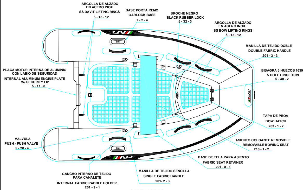
PLANT VIEW VISTA SUPERIOR
